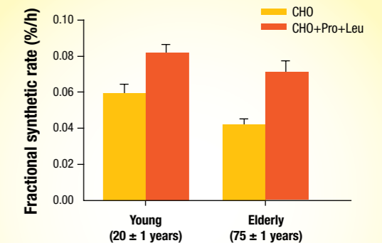
Figure 6. Protein and leucine co-ingestion with carbohydrates stimulates muscle protein synthesis in young and elderly men 4
