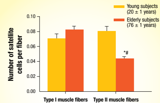
Figure 5. Atrophy of type II muscle fibres in the elderly but not the young 2
